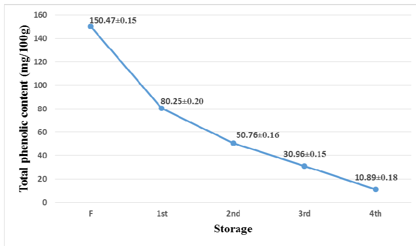
Figure 3. Changes in total phenolic content in the Palmyrah young fruit kernel during canning and storage period (mg/100g)
